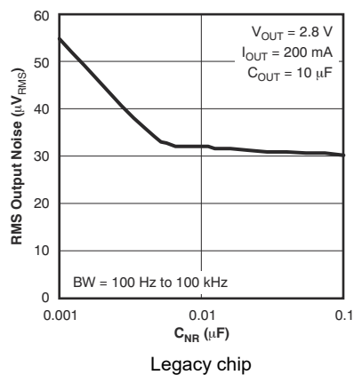
Figure 5-9. Root Mean Square Output Noise vs C_{NR}
