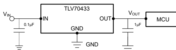
图 8-1. Typical Application
