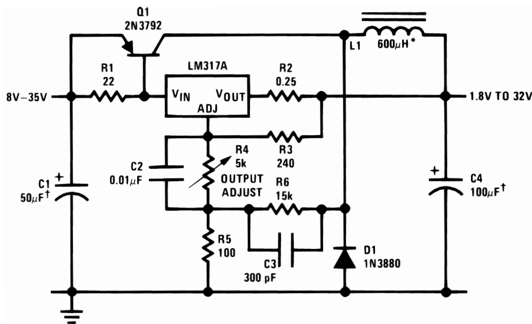
Figure 28. Low-Cost 3-A Switching Regulator
