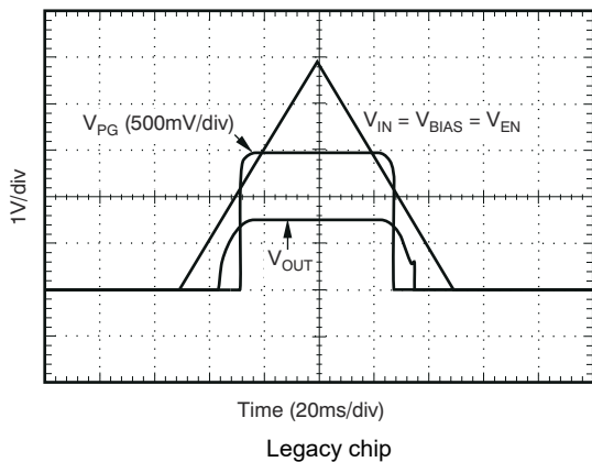
图 5-40. Power-Up, Power-Down
