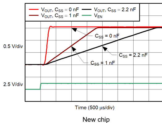
图 5-39. Turn-On Response
