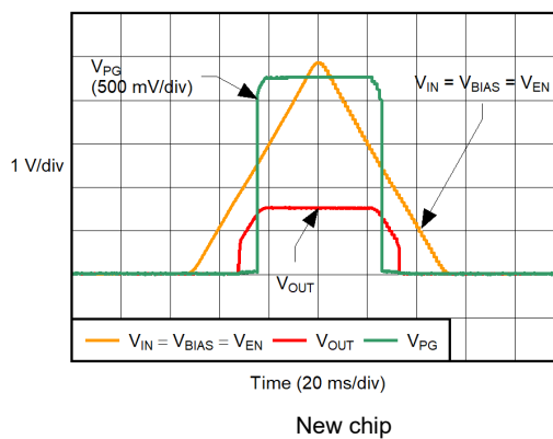
图 5-41. Power-Up, Power-Down
