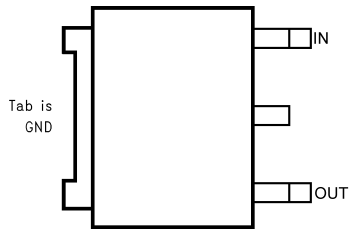
LP38690 TO-252 (NDP) 3 Pins Top View
