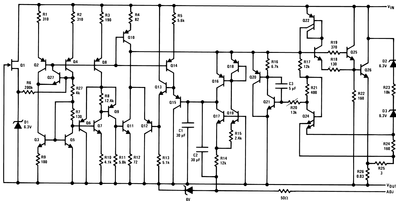
Figure 18. Schematic Diagram
